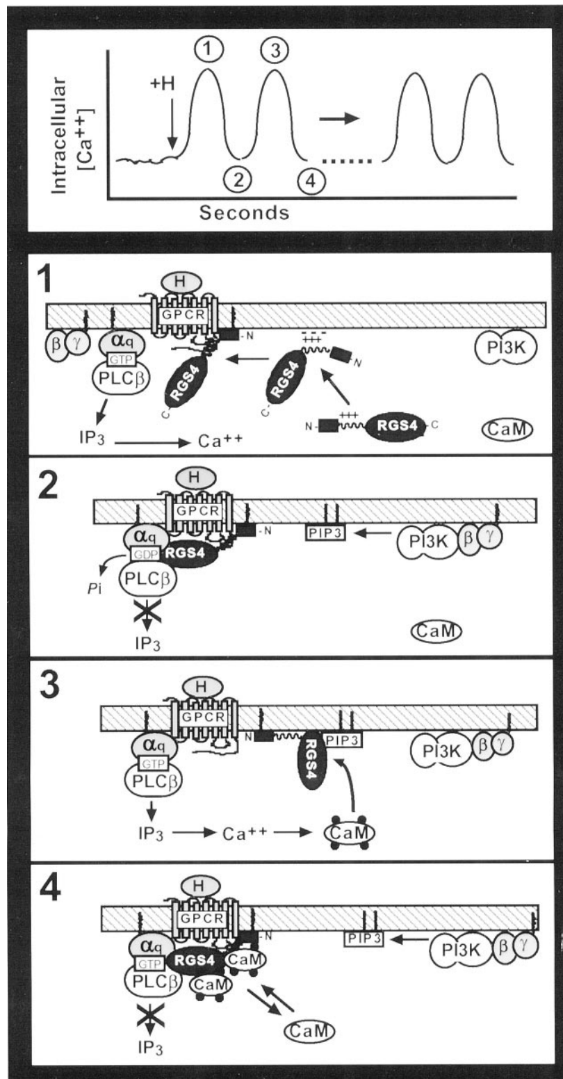
FIG. 2. Proposed model depicting RGS4 modulation of \text{Ca}^{2+} oscillations in mammalian cells. The following model is based on recently proposed ideas (Popov et al., 2000; Luo et al., 2001) and supporting data (see text and references therein). Top panel, schematic diagram illustrating peak amplitudes (1 and 3) and refractive periods (2 and 4) of rhythmic, oscillatory \text{Ca}^{2+} spikes in cells. Corresponding diagrams illustrating the proposed role of RGS4 in modulating each stage of the \text{Ca}^{2+} oscillations (1–4) are presented in panels 1–4. Panel 1, hormone (H) activation of GPCR stimulates the \text{G}_q/\text{IP}_3/\text{Ca}^{2+} pathway, resulting in RGS4 membrane recruitment and receptor association. Depicted are associations of the amphipathic helix on the N terminus of RGS4 (+++) with anionic lipids in the plasma membrane (- - -). Panel 2, RGS4 forms a complex with GPCR, \text{G}_q -GTP, and PLC \beta and exerts its GAP effects on \text{G}_q to shut off \text{Ca}^{2+} mobilization. \text{G}\beta\gamma activates PI3K, which synthesizes PIP _3 . Panel 3, PIP _3 binding to RGS4 inhibits its GAP activity toward \text{G}_q , allowing resumption of IP _3 production and \text{Ca}^{2+} mobilization. \text{Ca}^{2+} (●) activated CaM competes with PIP _3 for binding to RGS4. Panel 4, \text{Ca}^{2+} /CaM binding uncouples RGS4 from PIP _3 but does not inhibit RGS4 GAP activity. RGS4 reassociates with the \text{G}_q /GPCR complex to shut off IP _3 / \text{Ca}^{2+} production. As \text{Ca}^{2+} levels fall, CaM is deactivated and dissociates from RGS4, allowing rebinding of PIP _3 . See text for further discussion.
